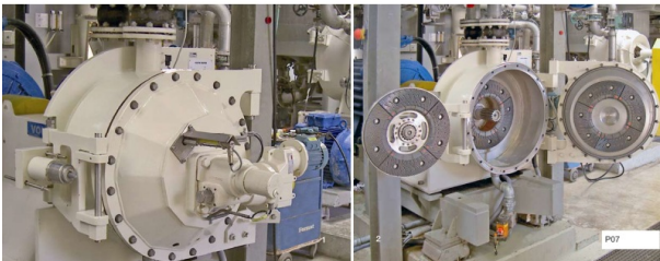
1 TwinFlo 2 TwinFlo opened, with PLURALIS fittings
